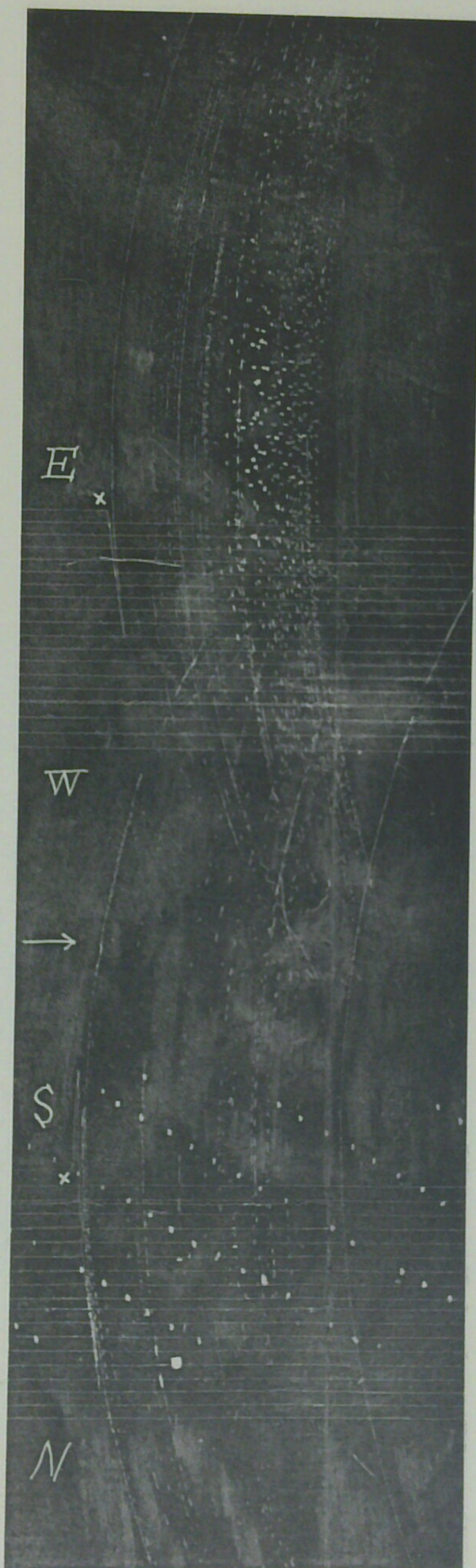
Fig. 9. The 2nd Destructive Omachi Earthquake, on Nov. 11, 1918, at 4.03 P.M. Horizontal Pendulum Tromometer Record at the Nágano Meteorological Observatory. Multiplication = 62.
