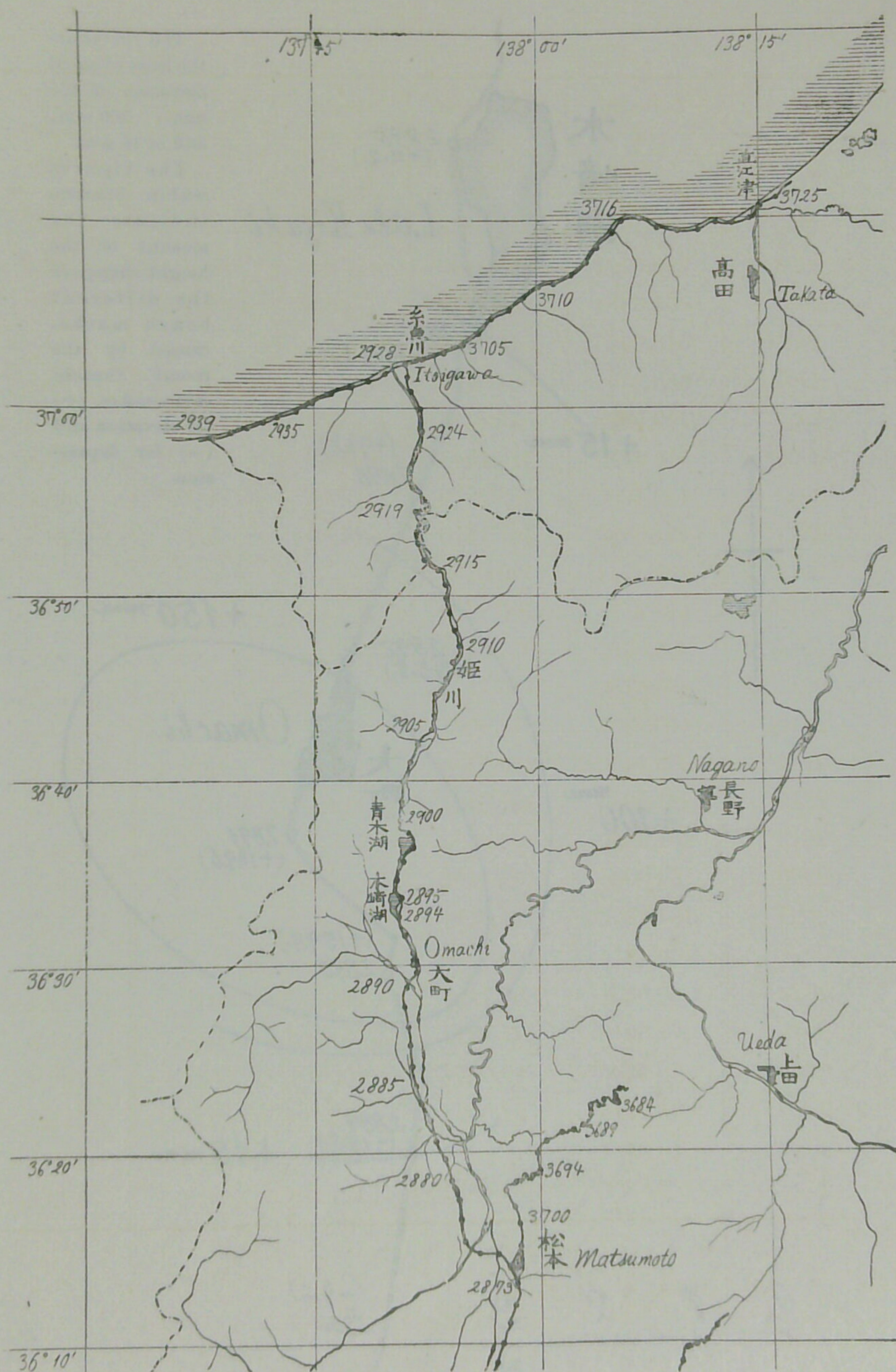
Fig. 20. Map showing the Precise Leveling Line between Matsumoto and Itoigawa and in the neighbouring regions.
