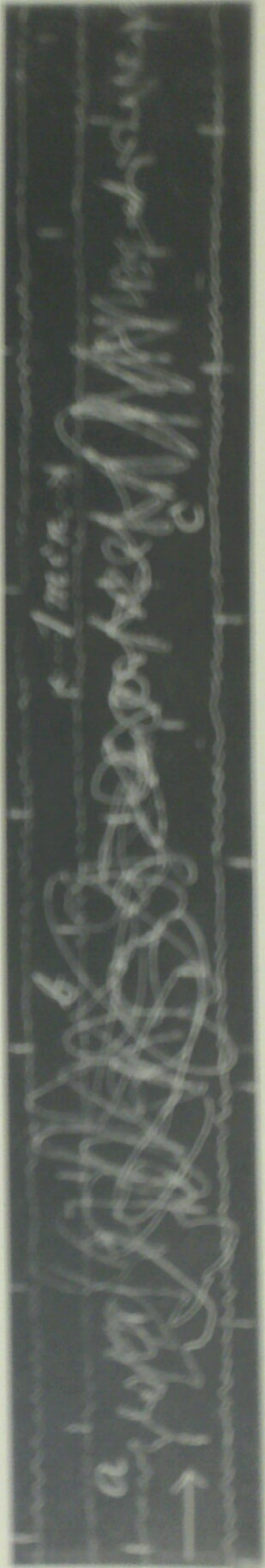
Fig. 3. The Strong Aftershock on Nov. 11, 1918, at 3.10 a.m.
