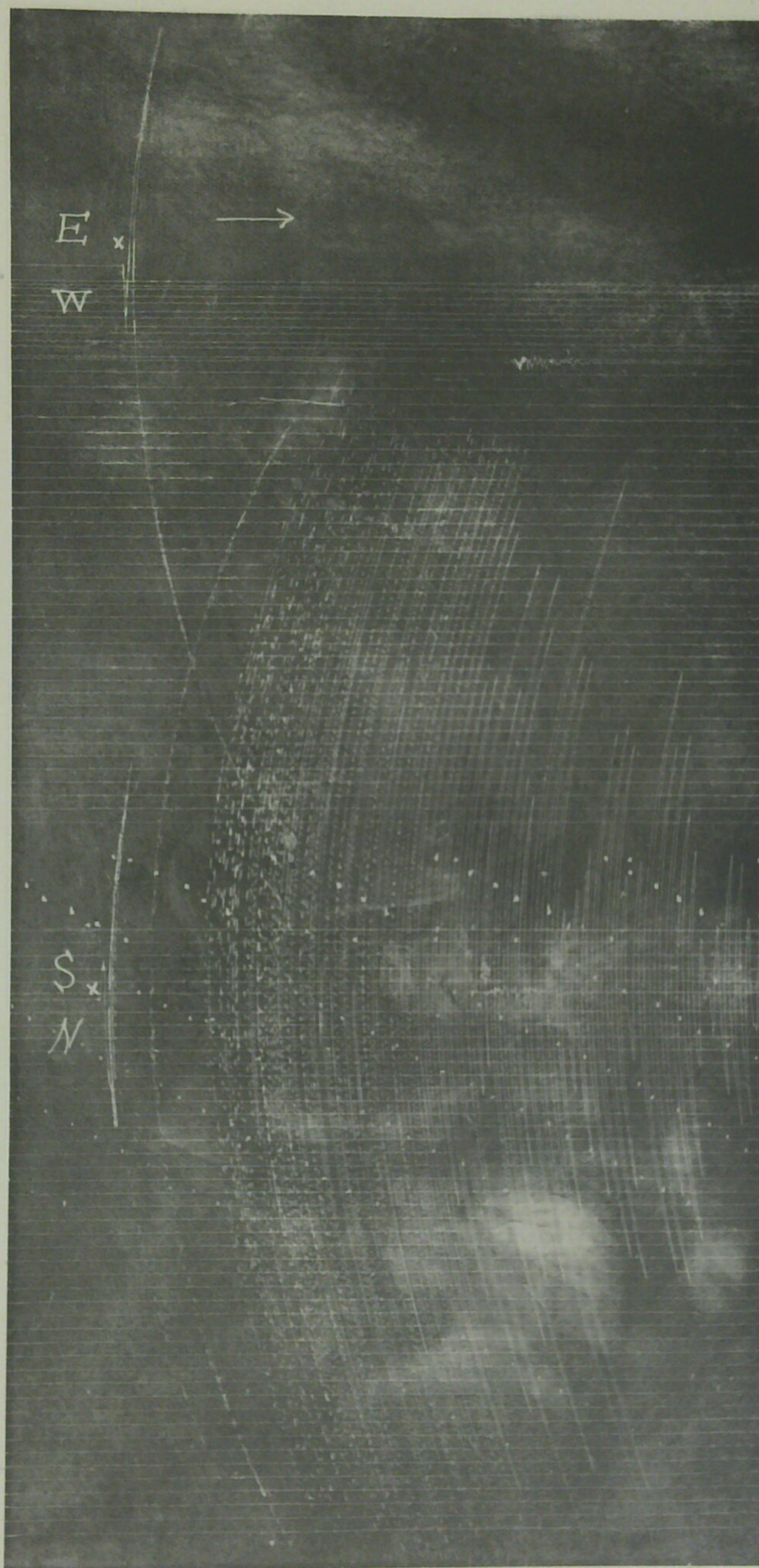
Fig. 10. The 1st Destructive Omachi Earthquake, on Nov. 11, 1918, at 2.58 A.M. Horizontal Pendulum Tromometer Record at the Nagano Meteorological Observatory. Multiplication = 60.
