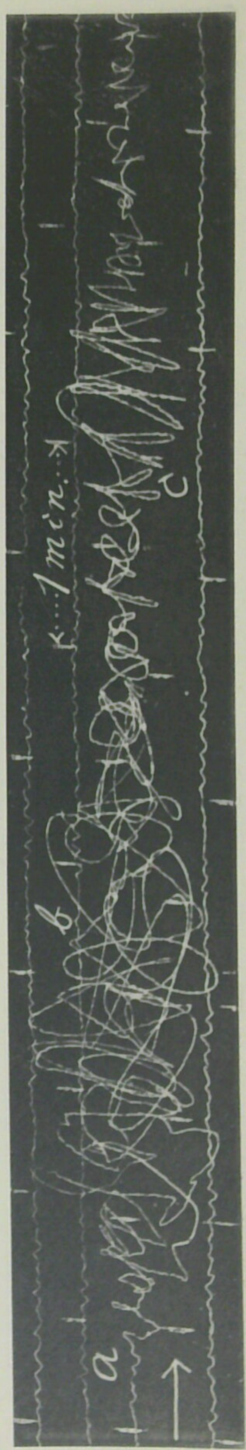
Fig. 8. The Strong Aftershock on Nov. 11, 1918, at 3.16 A.M.
