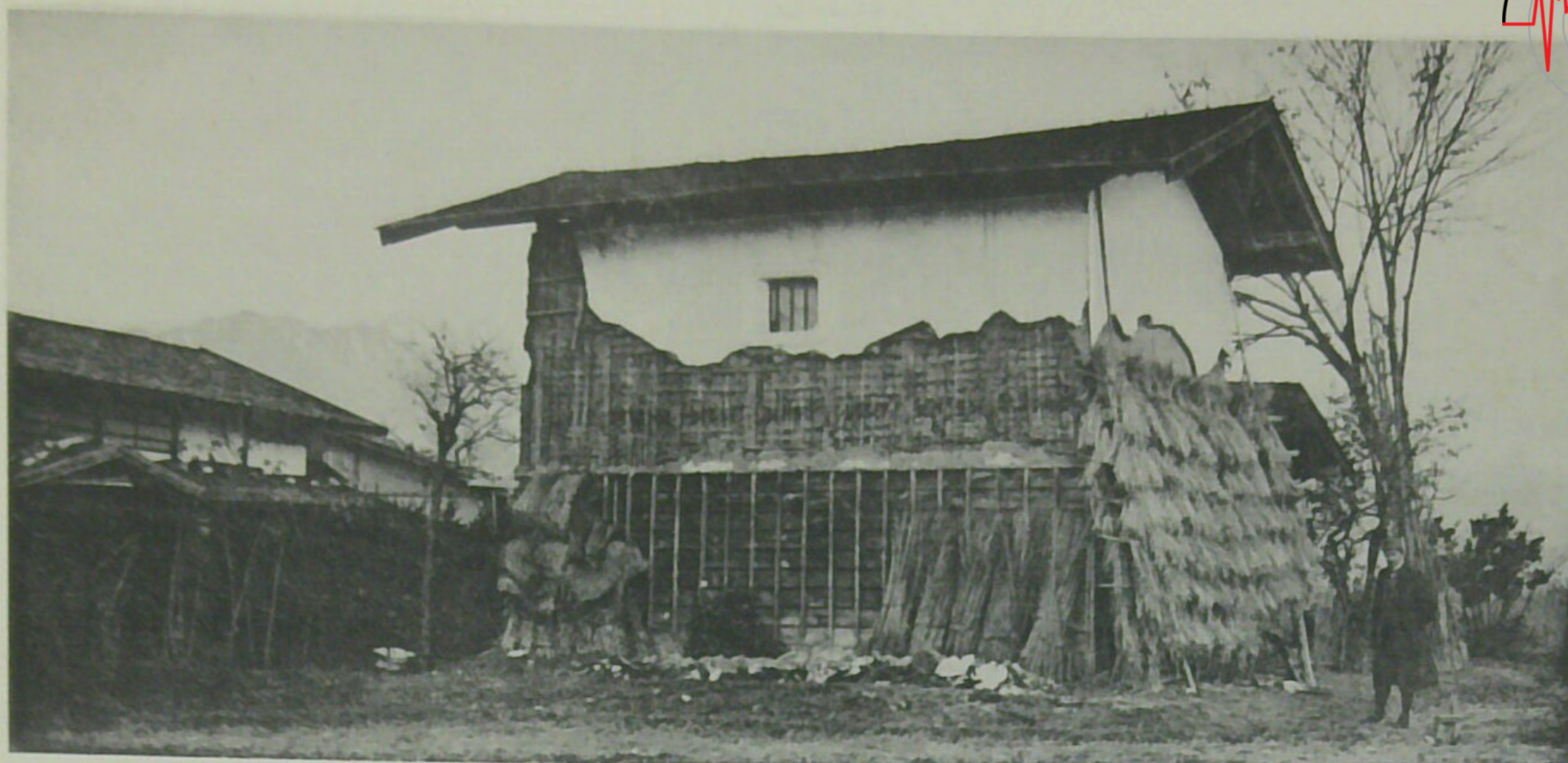
Fig. 3. A Dozo (Japanese Ware-house) at Shimizu, Tokiwa-mura, with its mud wall badly shaken down
