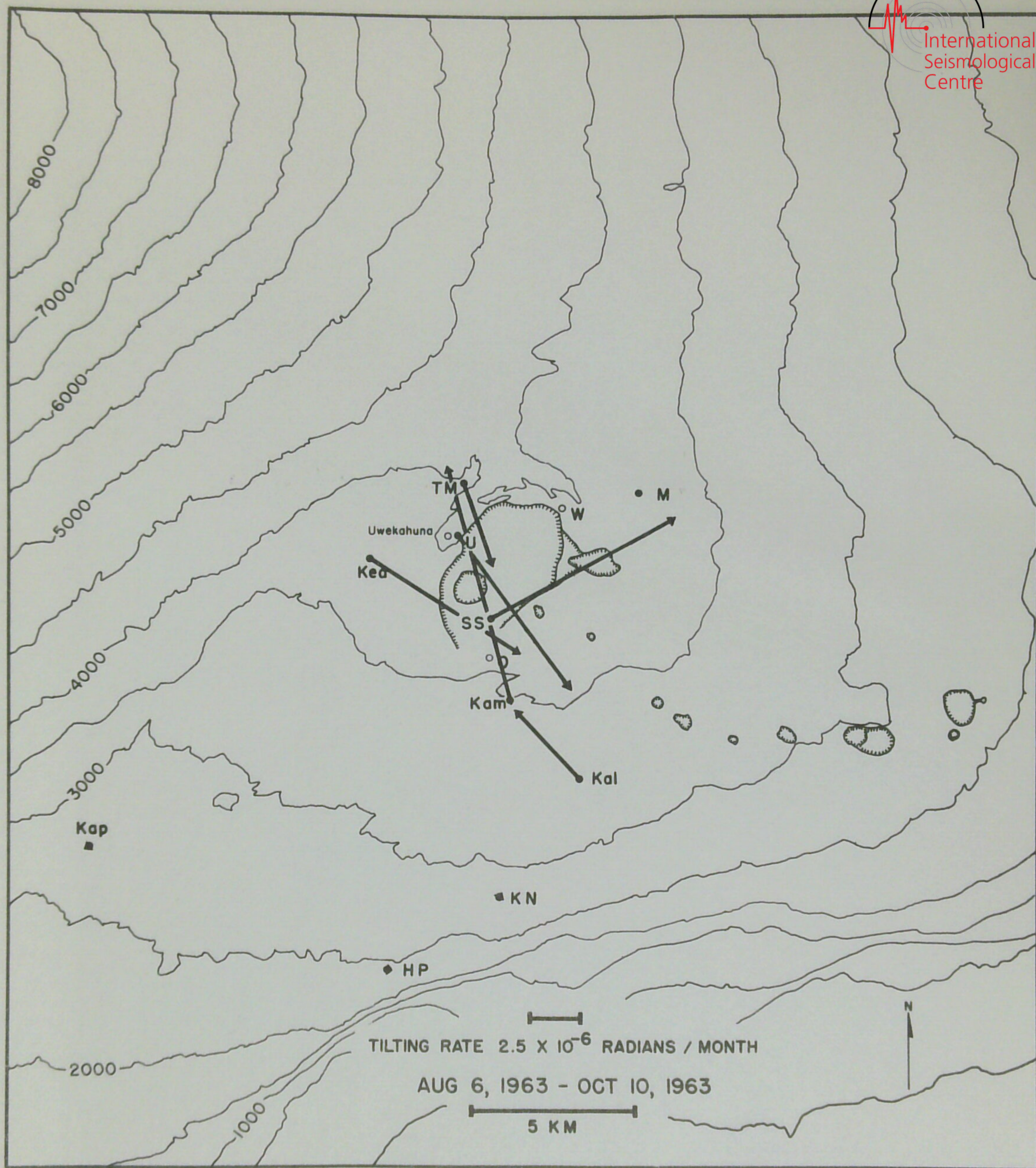
Figure 2.--Tilting of the ground around Kilauea caldera, August 6 to October 10, 1963. The vector depicting tilting at a given tilt base points in the direction of maximum relative subsidence and has a length proportional to the rate of tilting during the measurement interval. Closed circles represent field tilt bases; open circles, short-base water-tube tiltmeters.
